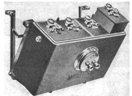
WORCESTER SWINGING SPARK COIL.
